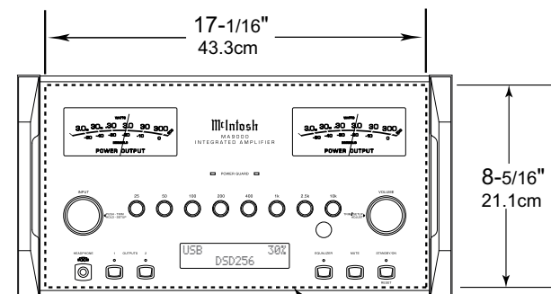
Cutout Opening for Custom Mounting
