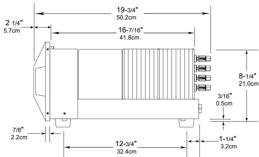
Side View of the MA9000
