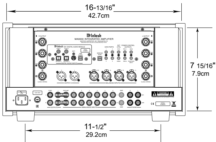
Rear View of the MA9000
