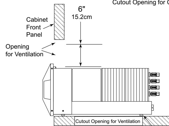
Cutout Opening for Custom Mounting
