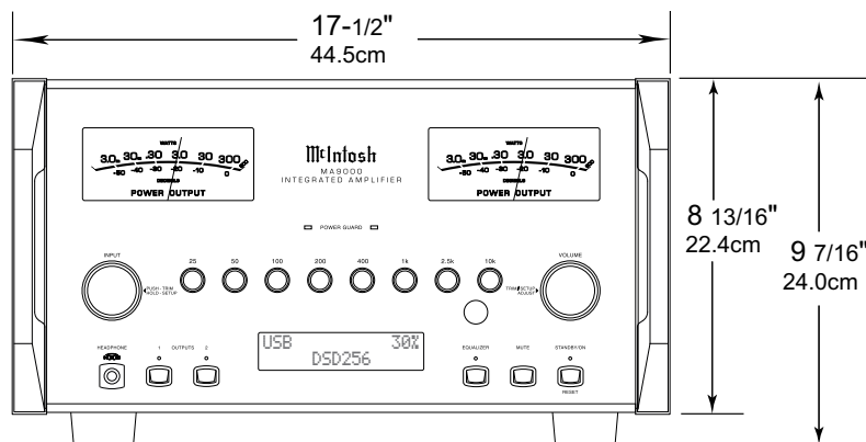
Front View of the MA9000
